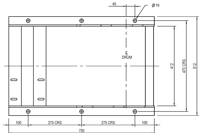
SECTION A-A MOUNTING DETAIL
